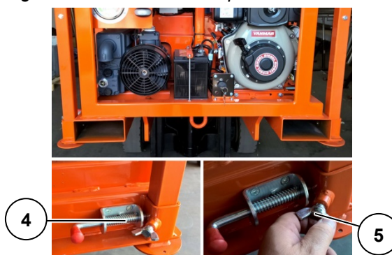
Figure 7 : Position de transport
