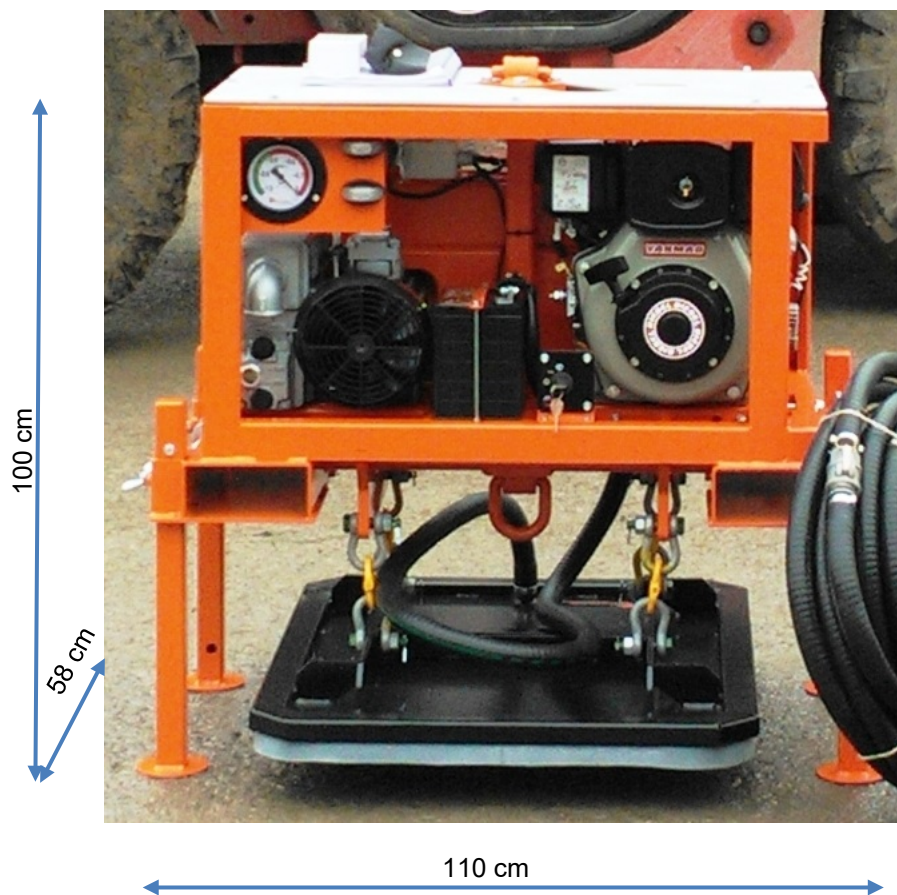
Figure 3 : Dimensions
